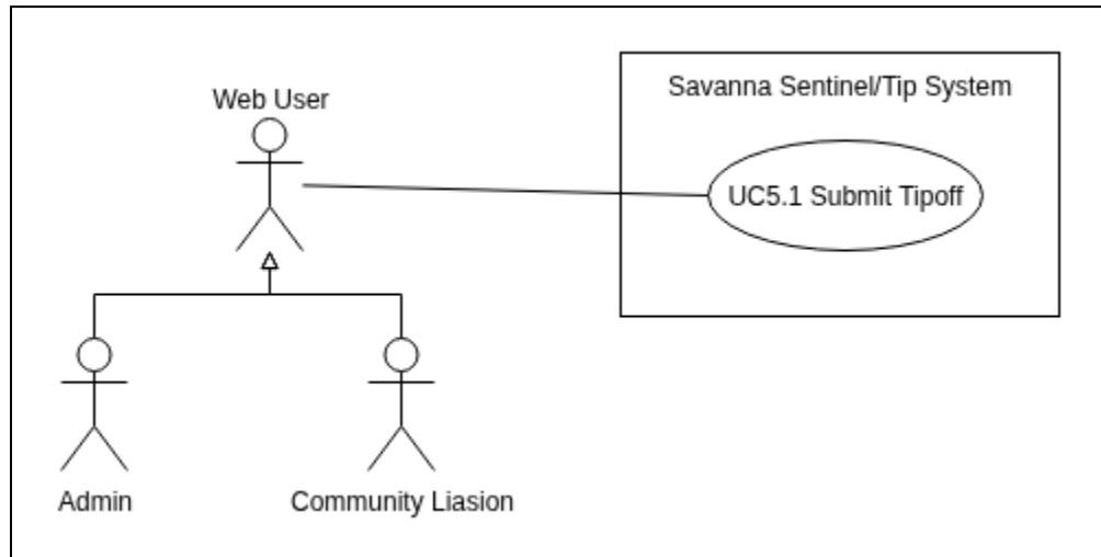
Figure 5 - Tip-off Subsystem
