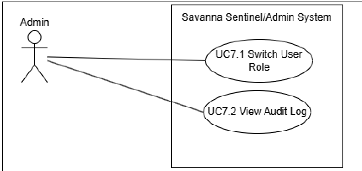
Figure 7 - Admin Subsystem
