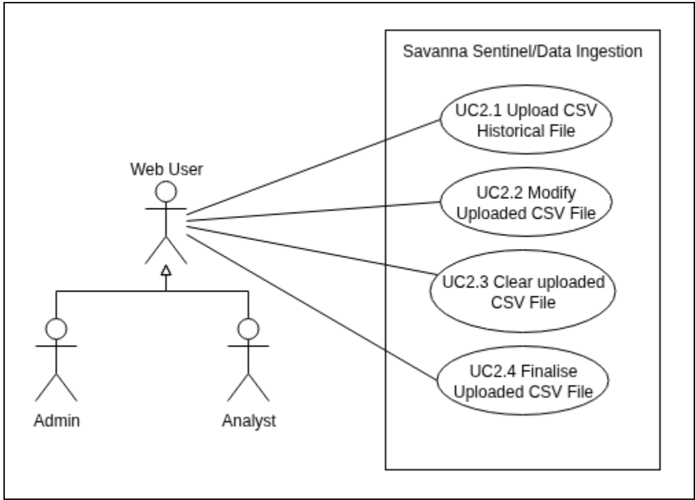
Figure 2 - Ingestion Subsystem
