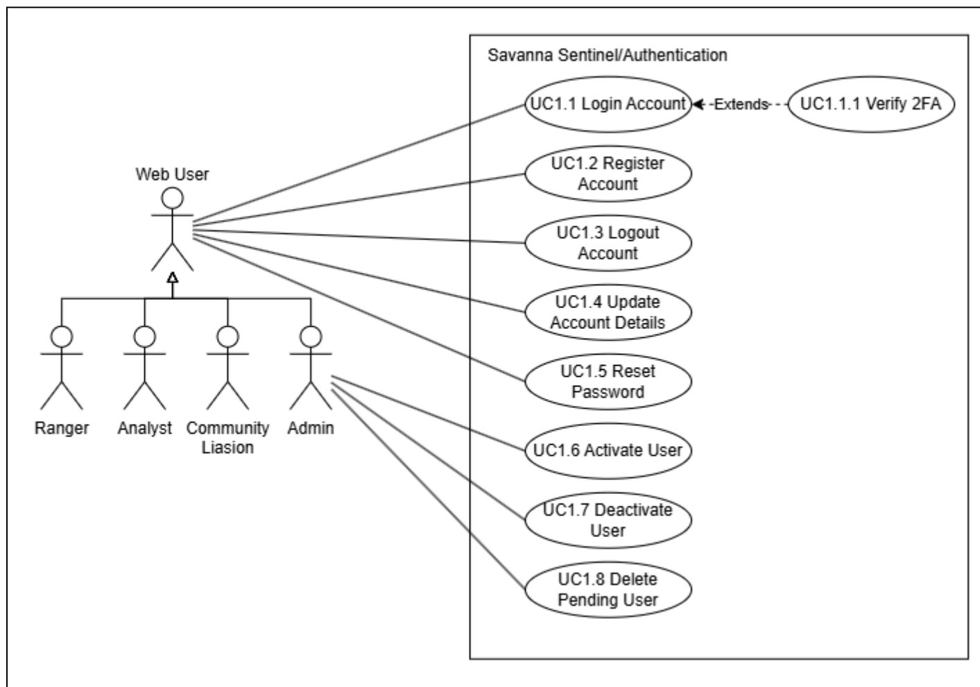
Figure 1 - Authentication Subsystem
